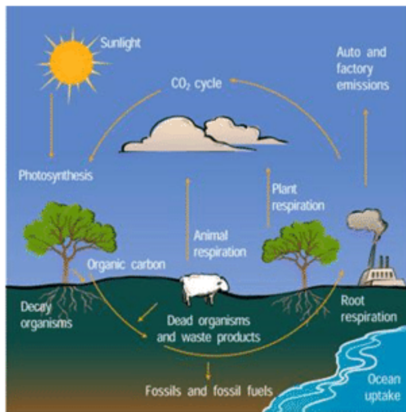
The carbon cycle
